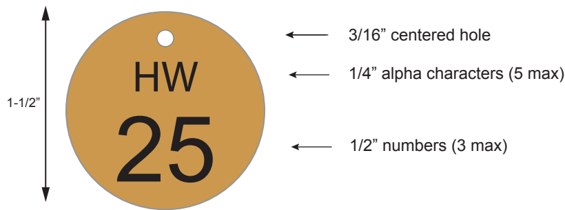
Dimension: 1-1/2" Sq.
