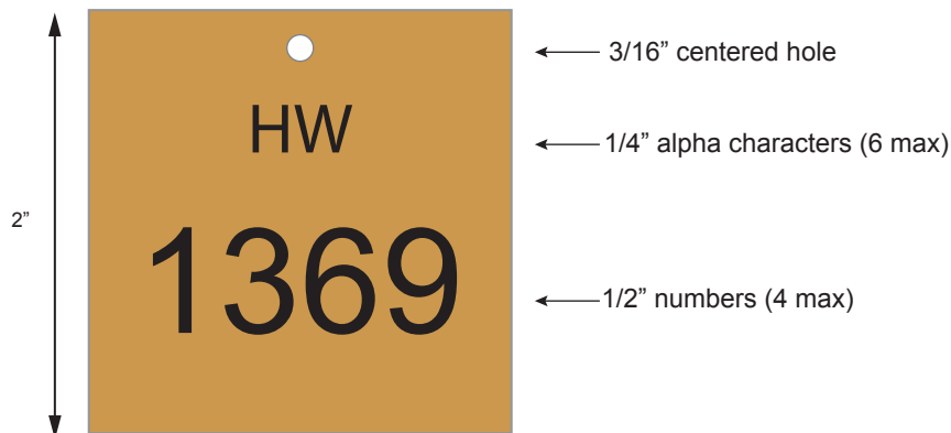
Dimension: 2" Sq.
